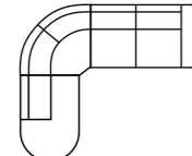
Round open corner (L) Art. No.: 12040 A-H86 x D259 x W278cm B-H86 x D259 x W288cm
